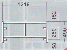
WF8 LADDER FRAME
