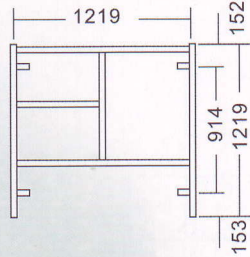
WF9 HORIZONTAL FRAME
