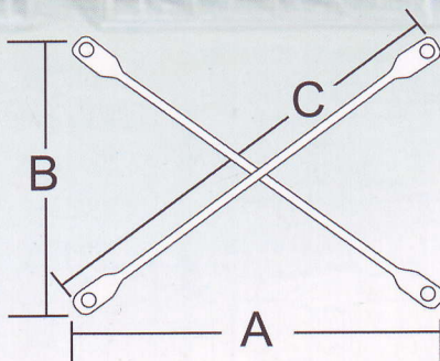
Cross Braces
