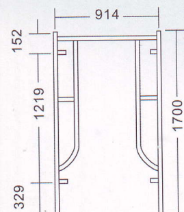
WF4 MAIN FRAME
