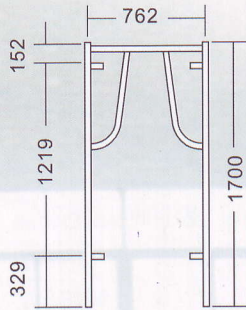
WF5 MAIN FRAME
