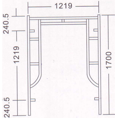
WF1 MAIN FRAME
