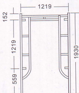
WF2 MAIN FRAME
