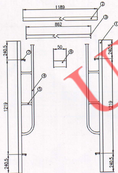
WF2 MAIN FRAME
